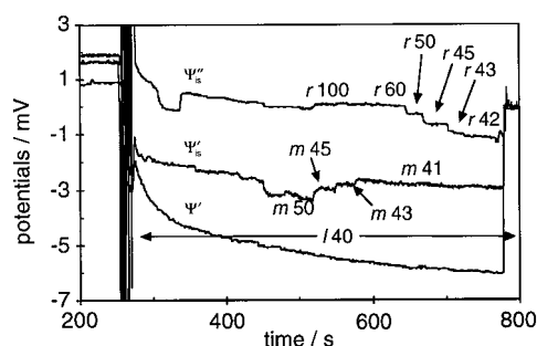
FIGURE 2 Bottom trace: potential between the Ag/AgCl electrodes; middle trace: the ISM' potential from the left, closed compartment (''); top trace: potential from the ISM'' in the right, open compartment (''). The left microelectrode was positioned at 40 on the graticule (1 unit = 25 \mu\text{m} ) immediately after the addition of urea and held at 40. Between 400 and 600 s the membrane position was adjusted to the values shown to obtain a profile of potential in the closed compartment (graticule positions prefixed by m ). Between 620 s and membrane breakage the position of the right microelectrode was adjusted to obtain a profile in the open compartment. At 780 s the membrane was broken using a suction microelectrode. The potential traces have been offset to superimpose after membrane breakage when the two ISMs are recording the same potential and ion activity.
