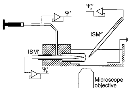
FIGURE 1 Experimental cell. \Psi' is the potential of the Ag/AgCl tube with respect to the Ag/AgCl earth wire. \Psi'_{is} and \Psi''_{is} are the potentials of the liquid ion exchanger microelectrodes (ISMs). The left, singly primed compartment is closed by the membrane, the seal around the microelectrode and the piston of the syringe are used to position the membrane. The right, doubly primed compartment is open. The entire cell is mounted on the stage of an inverted microscope.
