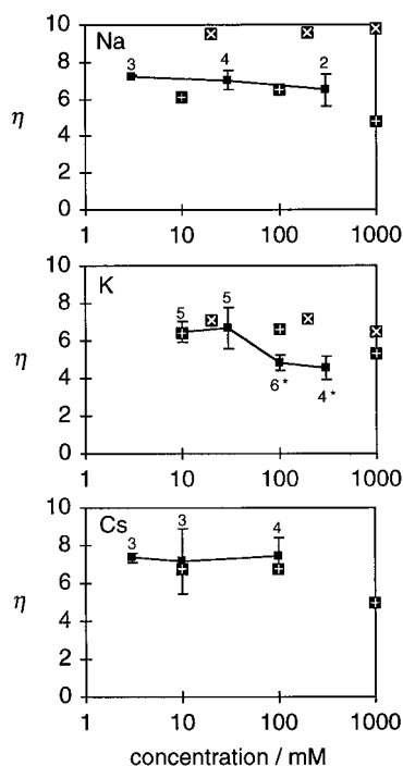
FIGURE 3 The number of water molecules transported per cation in gramicidin channels. Top, \text{Na}^+ ; middle, \text{K}^+ ; bottom, \text{Cs}^+ . ■, Error bars and connecting lines: data of the present study presented as mean \pm SE. The numbers near the error bars indicate the number of experiments. ✕, Values reported by Levitt (1984). +, Values reported by Rosenberg and Finkelstein (1978).
